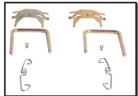
Disc Brake Hardware Kit #084-1250 Saab 99 (75- 80) and Saab 900 (79-87)
